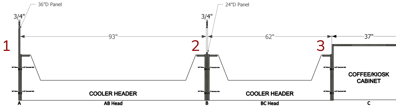
1 - End Panel to the End of a Bank Example
