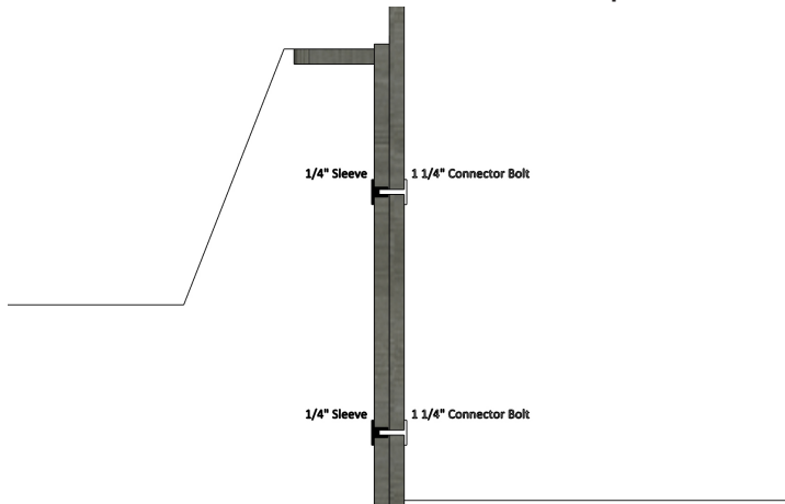
3 - Cooler Header to Cabinet Connection Example
