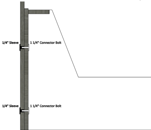
1 - End Panel to the End of a Bank Example
